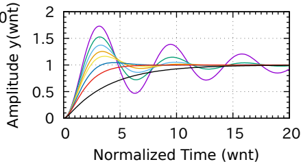
Second Order System - Unit Step Response
