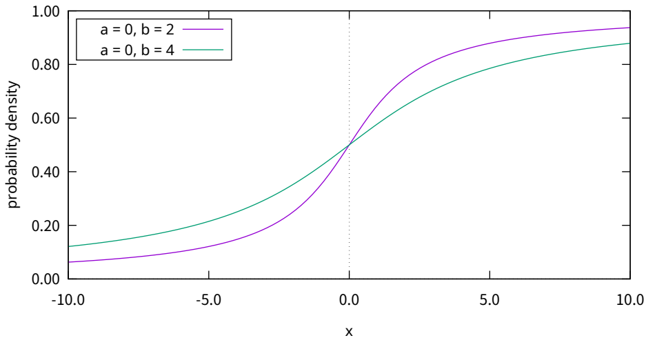
Cauchy CDF
