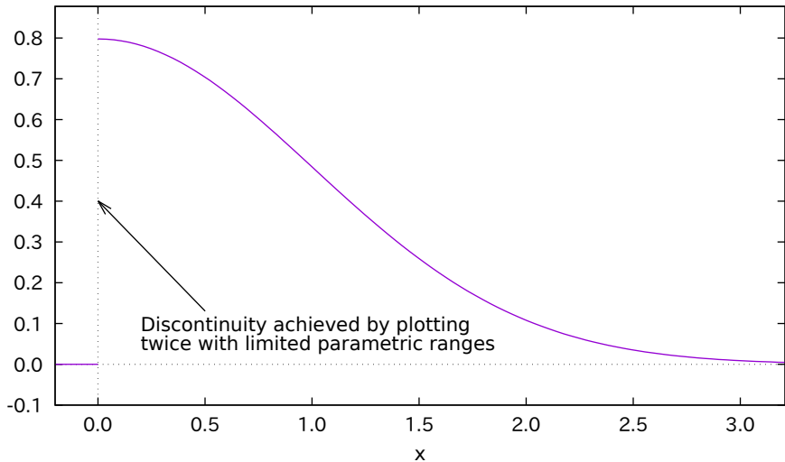
half normal PDF, \sigma = 1.0
