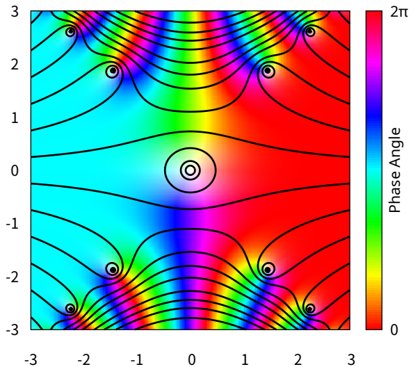
Complex error function \operatorname{erf}(x + iy)
