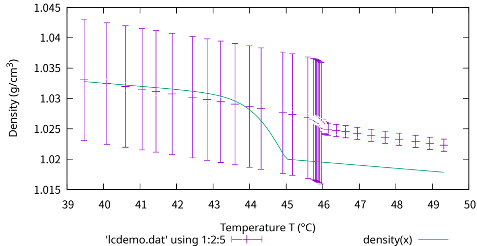
initial parameters for realistic model function
