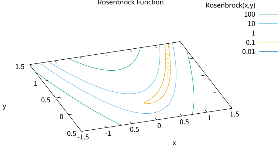
Rosenbrock Function
